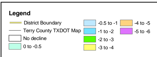
2003-2004 Change in Static Water Level Measurements (ft of change)
